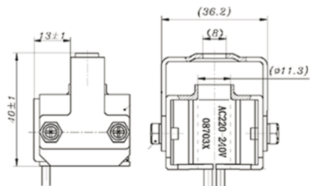
Drawing 2: FQA-55007
